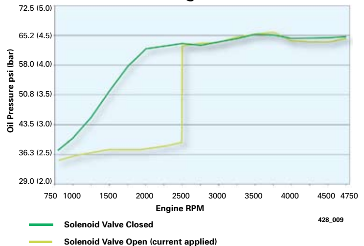
Oil Pressure Curve @ 212°F (100°C)
