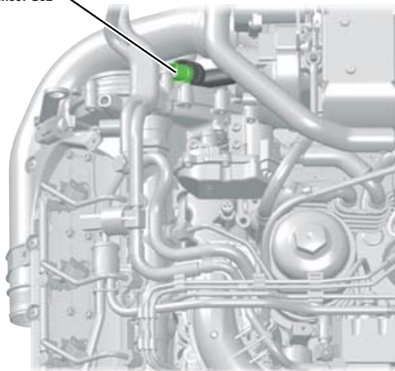
Engine Coolant Temperature (ECT) Sensor G62
