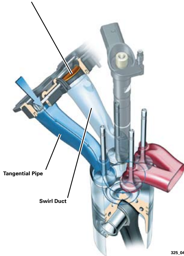
Butterfly Valve Closed
