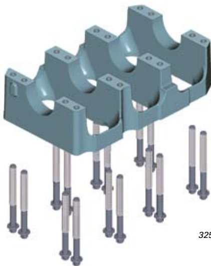
Bolts/Main Bearing Assembly
