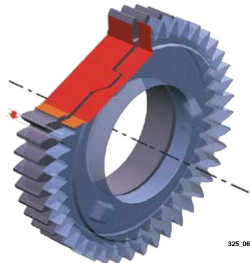
Clearance Compensation
