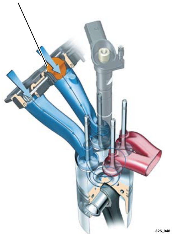
Butterfly Valve Open
