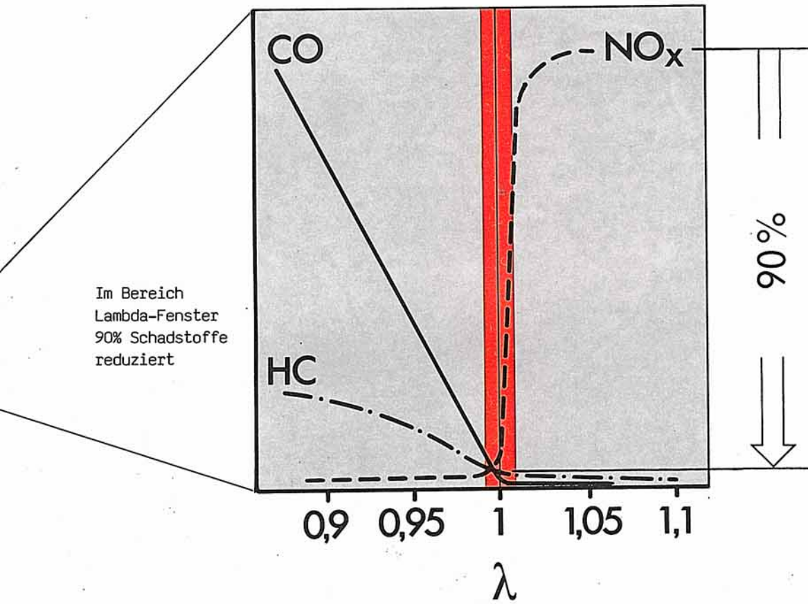
Lambda-Fenster
